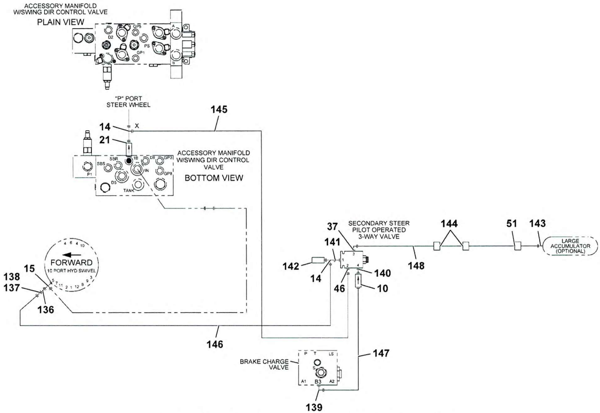
EMERGENCY FRONT STEER FOR CE CONFORMITY HYD LINES
