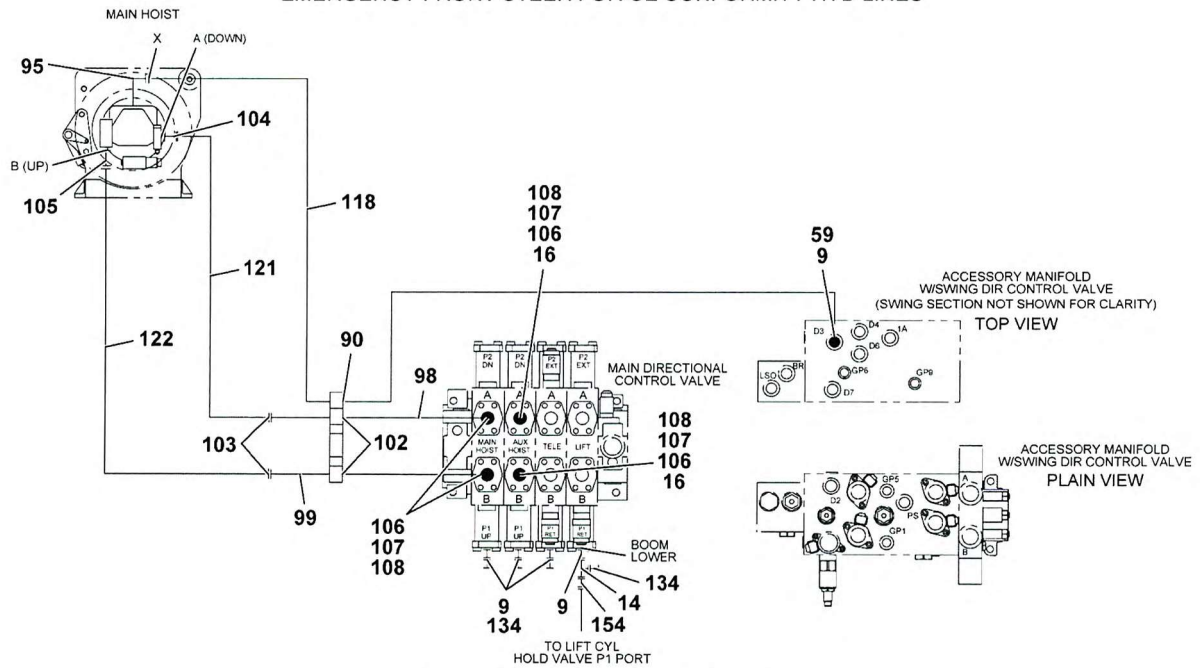
MAIN & FUTURE AUX HOIST HYD LINES
